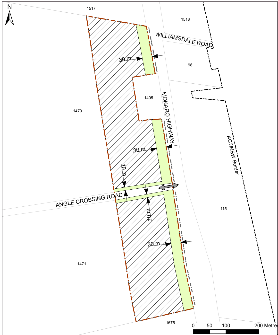
FIGURE 2 – DCP DRAWING 12/07
