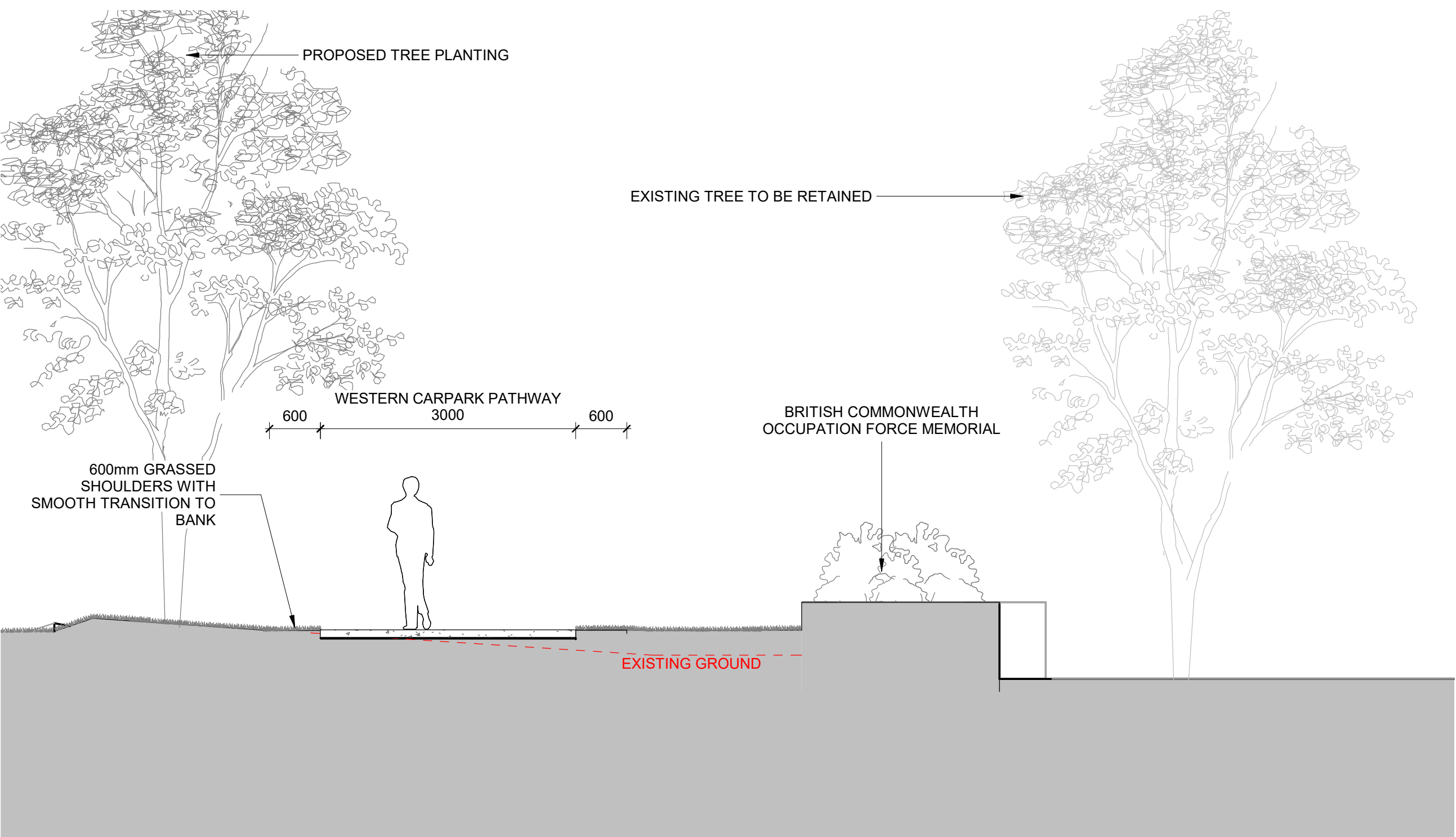
2 WESTERN CARPARK - MAIN PATHWAY INTERFACE WITH BCOF MEMORIAL 1 : 50
