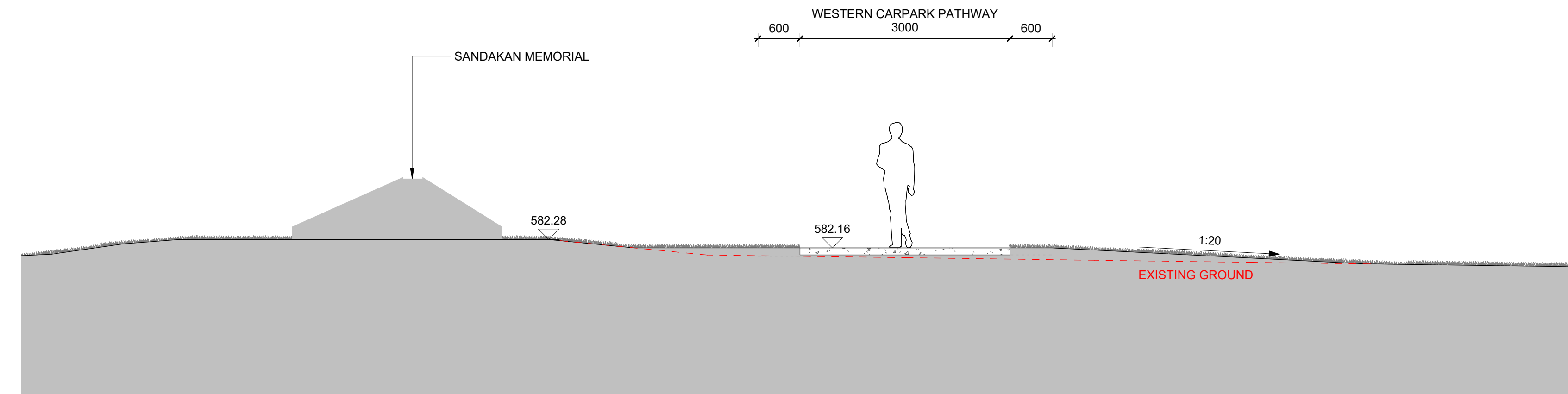
4 WESTERN CARPARK - MAIN PATHWAY INTERFACE WITH SANDAKAN MEMORIAL 1 : 50
