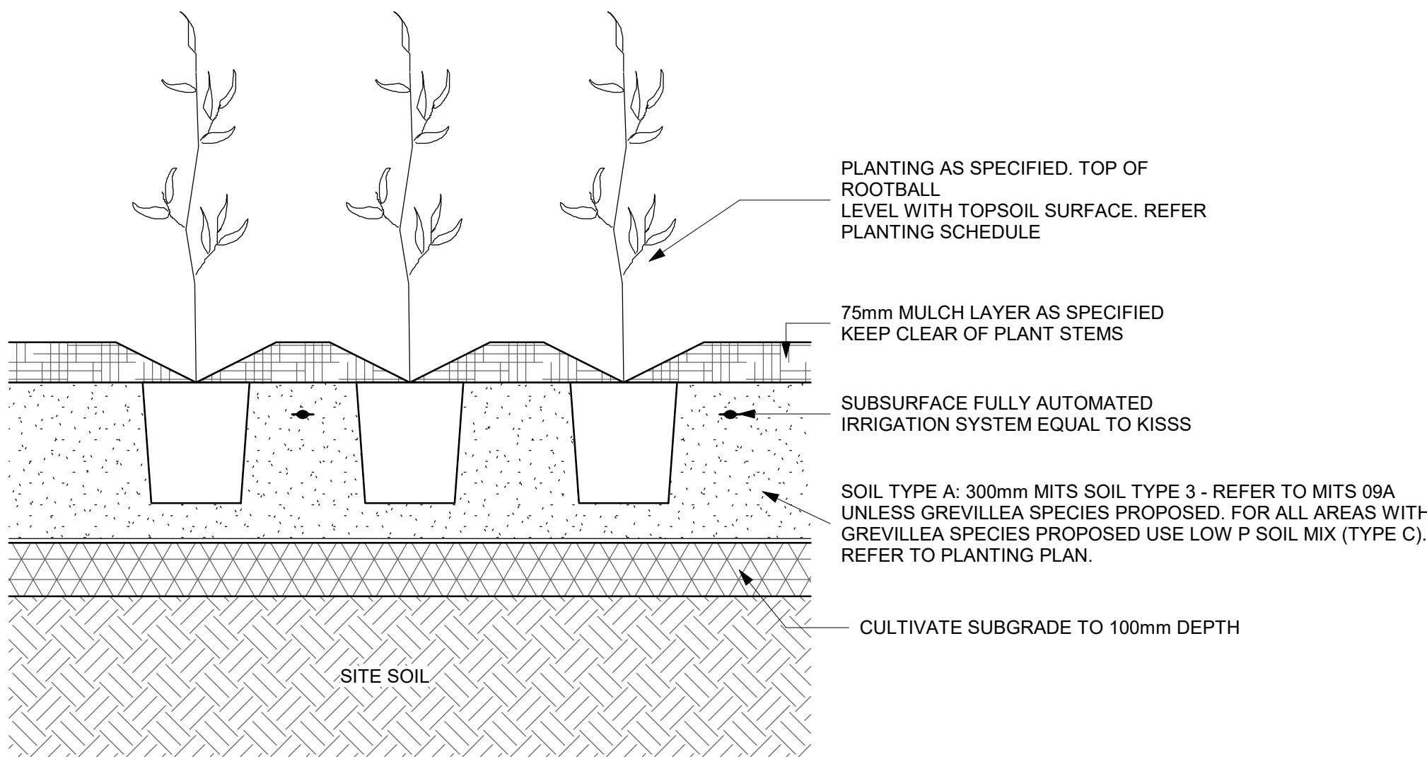
4 TYPICAL PLANTING DETAIL 1 : 10
