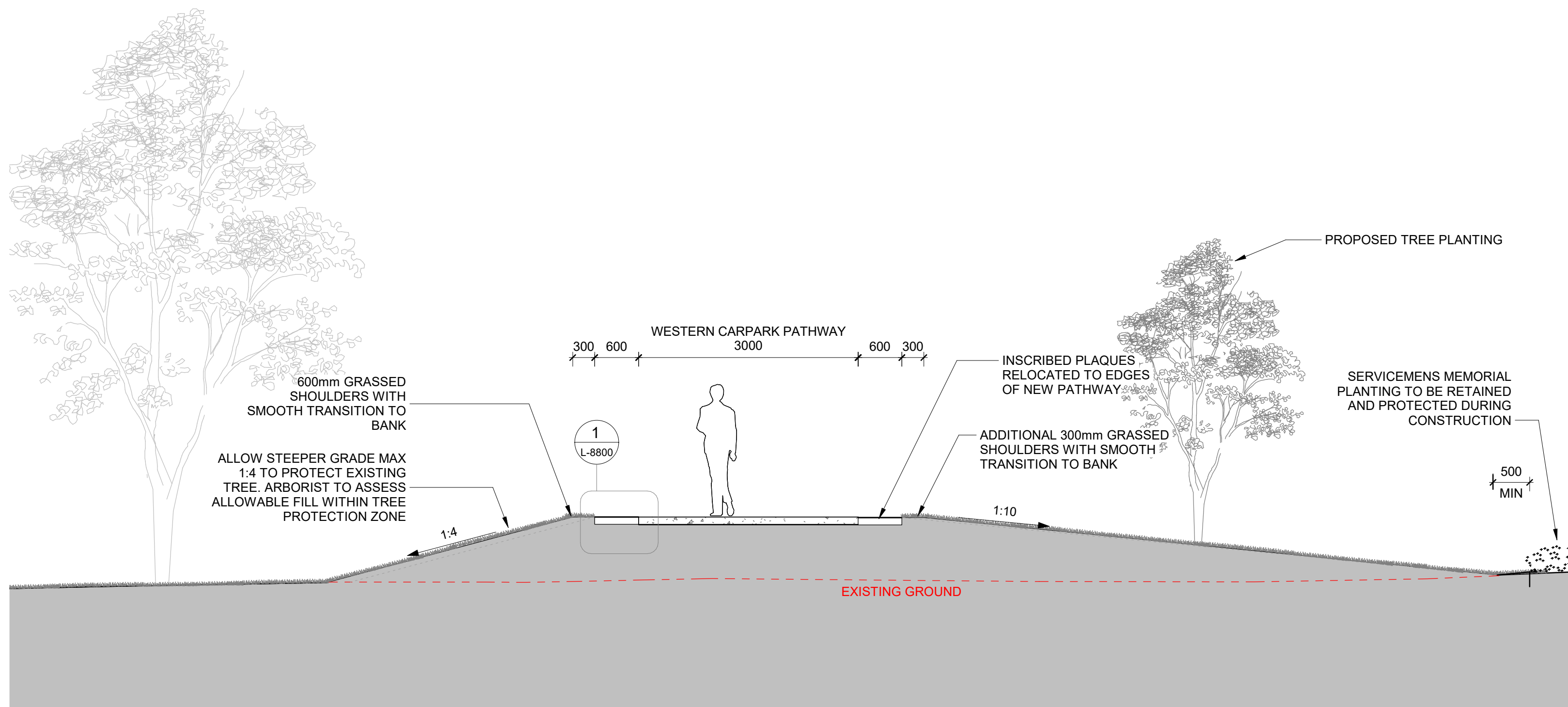
1 WESTERN CARPARK - MAIN PATHWAY TYPICAL 1 : 50
