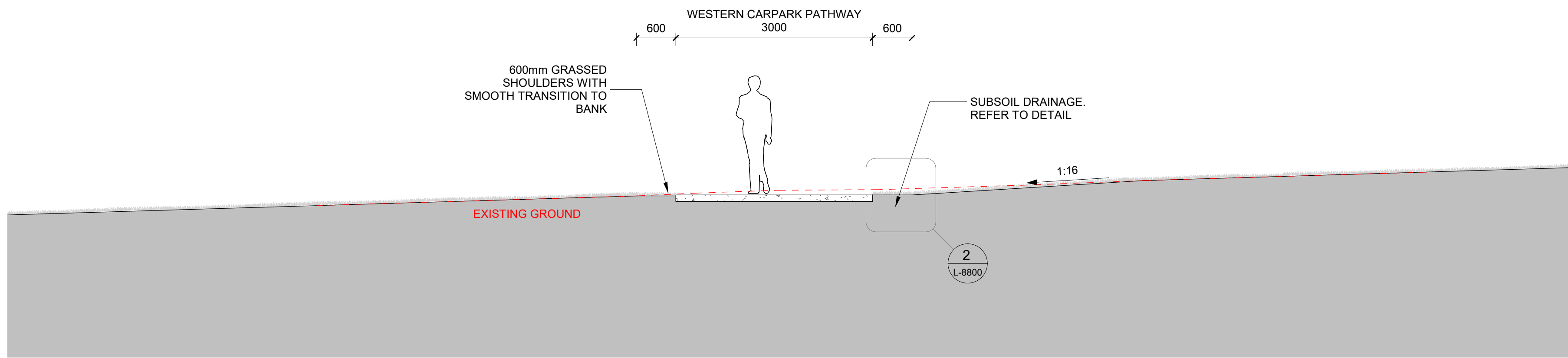
3 WESTERN CARPARK - MAIN PATHWAY AND SUBSOIL DRAINAGE SYSTEM 1 : 50
