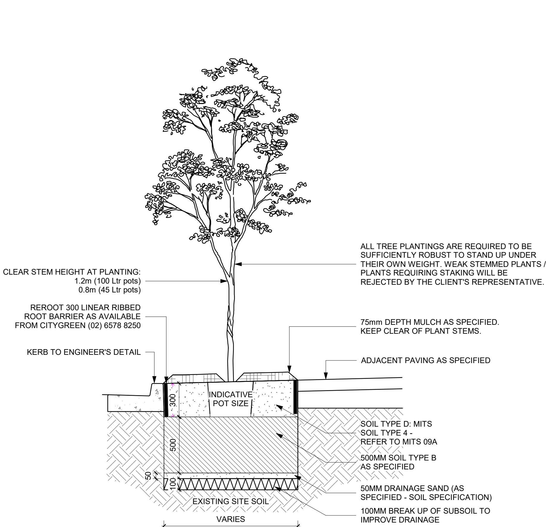
3 TYPICAL TREE PLANTING DETAIL IN CARPARK 1 : 20
