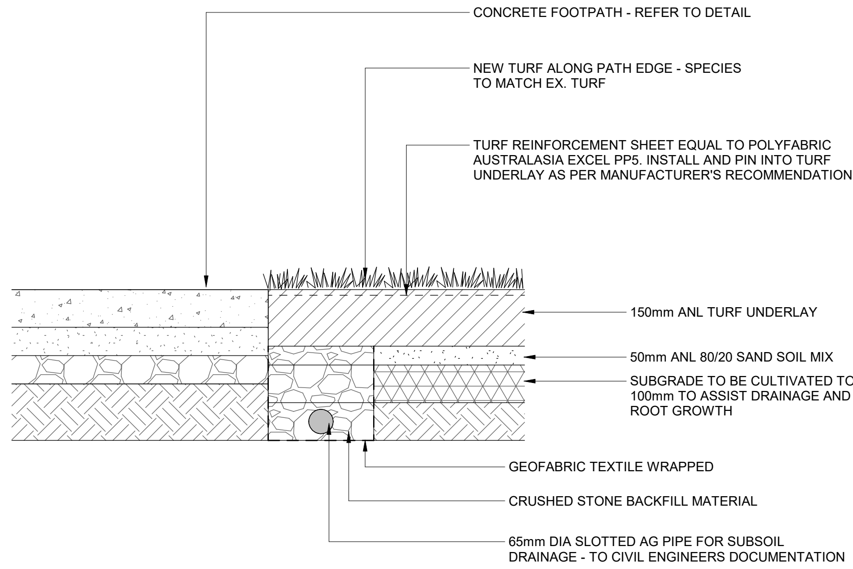
2 SUBSOIL DRAINAGE SYSTEM DETAIL 1 : 10
