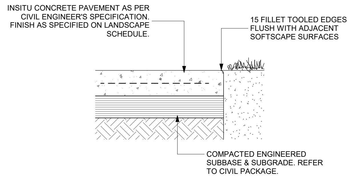
5 PV1 -TYPICAL CONCRETE INSITU PAVING 1 : 10
