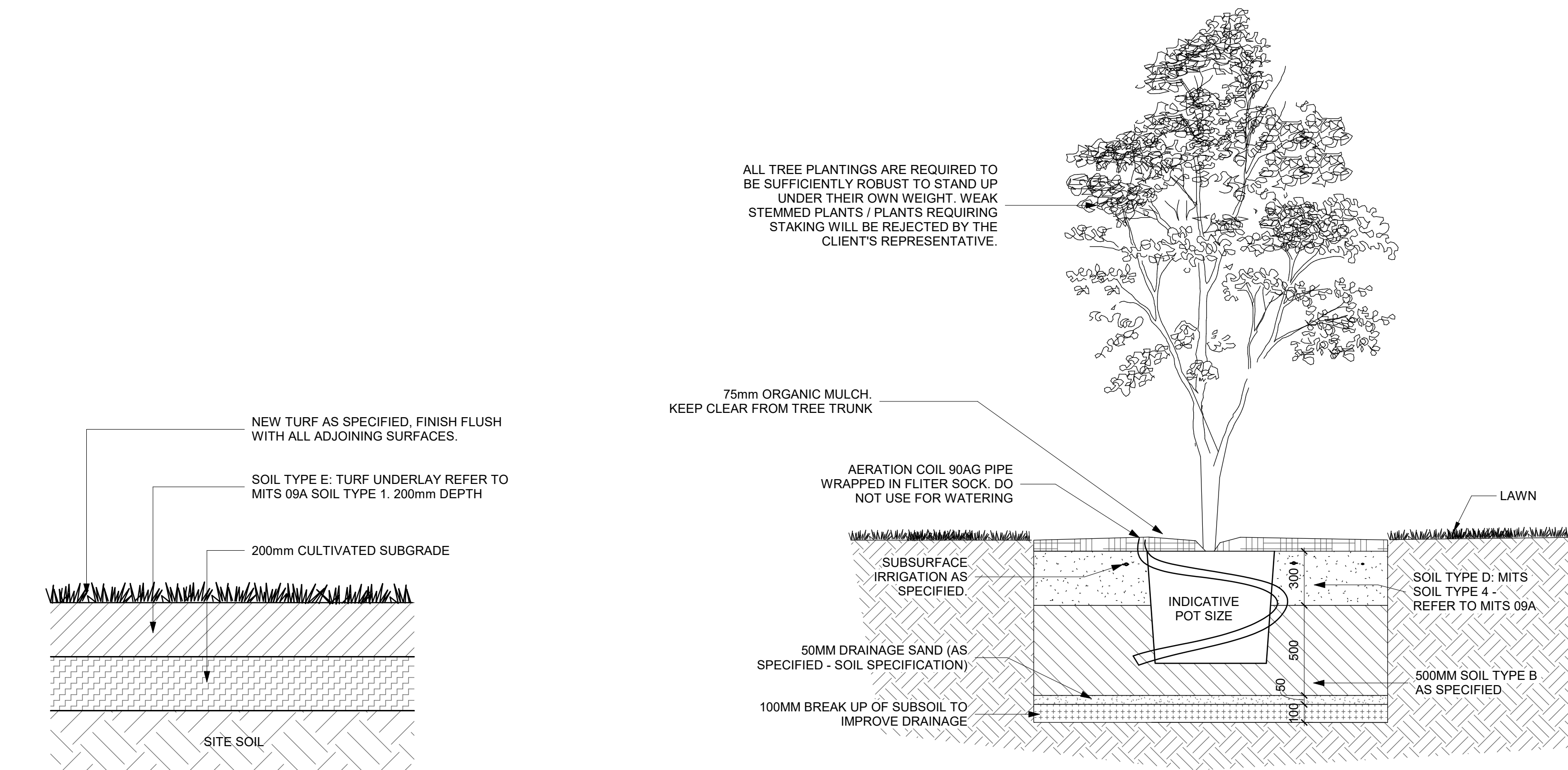
1 TYPICAL LAWN DETAIL 1 : 10
