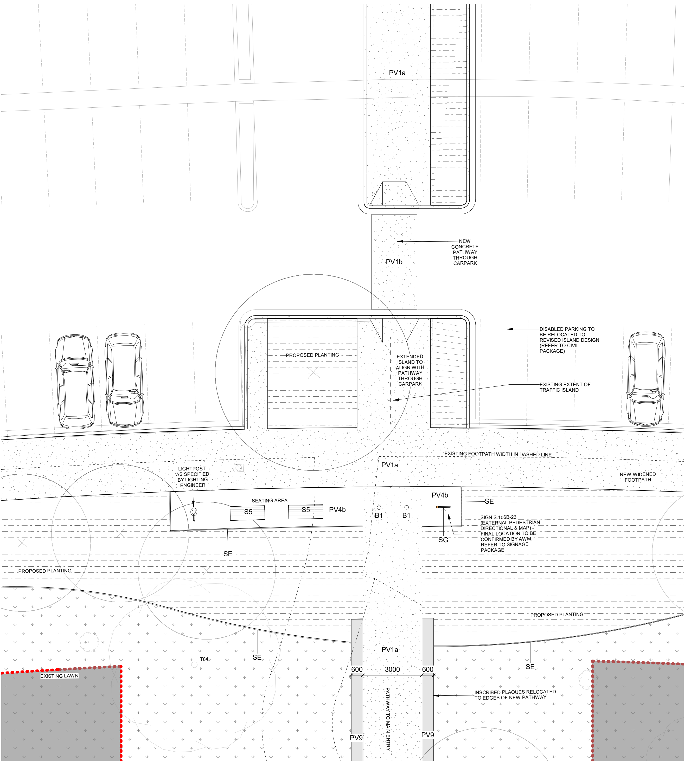
1 PATHWAY ENTRY DETAIL 1 : 100
