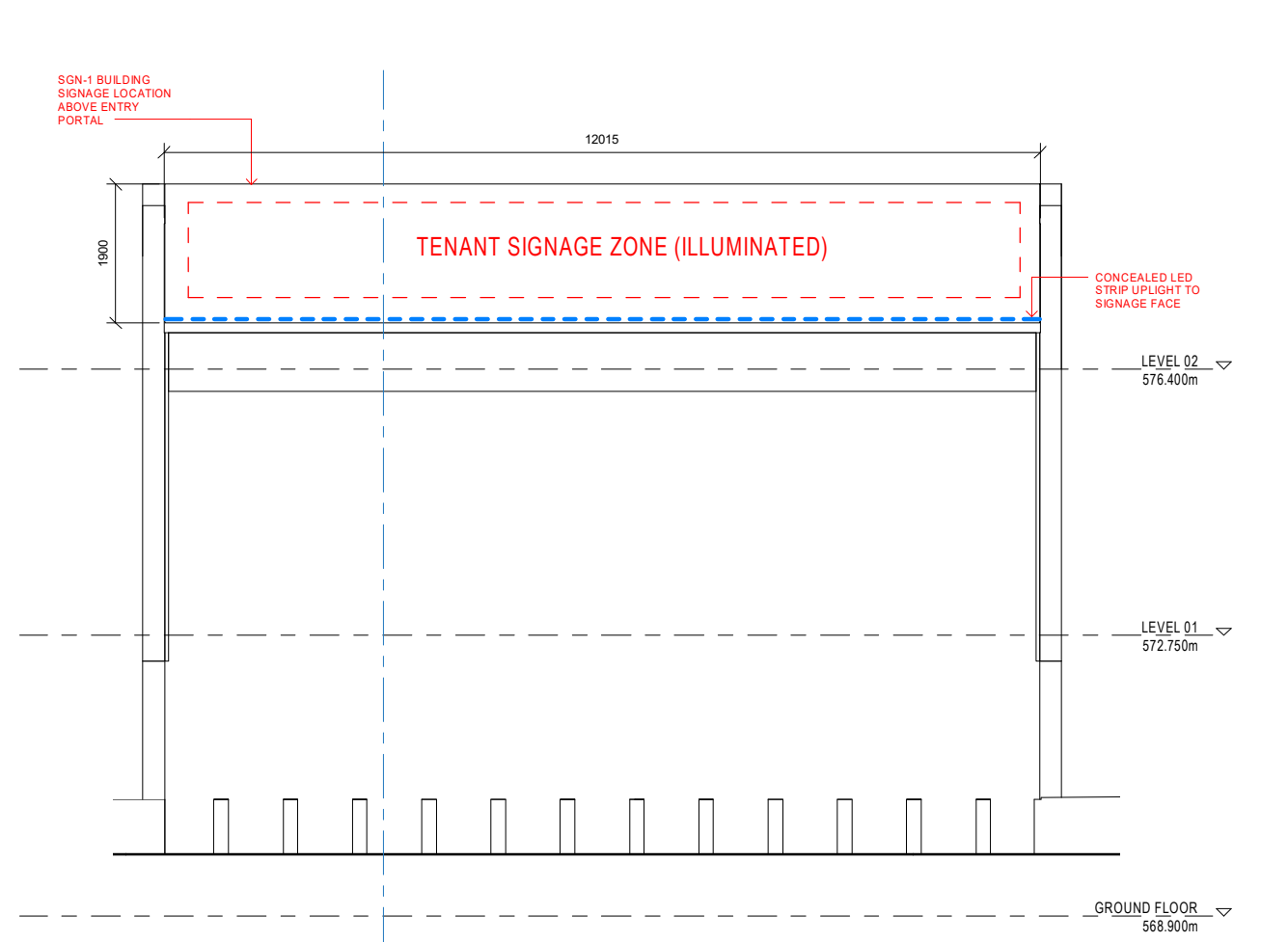
1 SGN-1 FRONT ELEVATION
