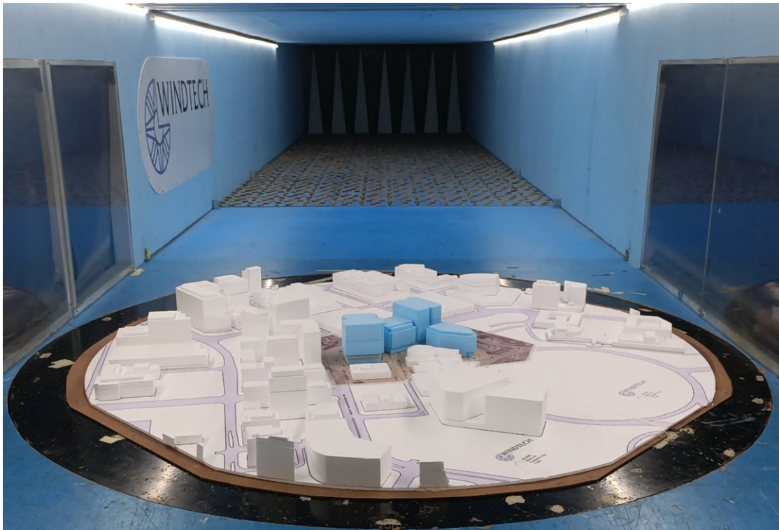
Figure 1d: Photograph of the Wind Tunnel Model (view from the south-west)
