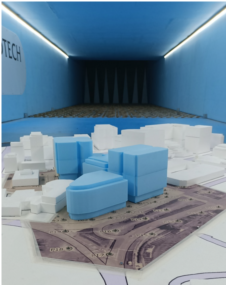
Figure 1a: Photograph of the Wind Tunnel Model (view from the south-east)
