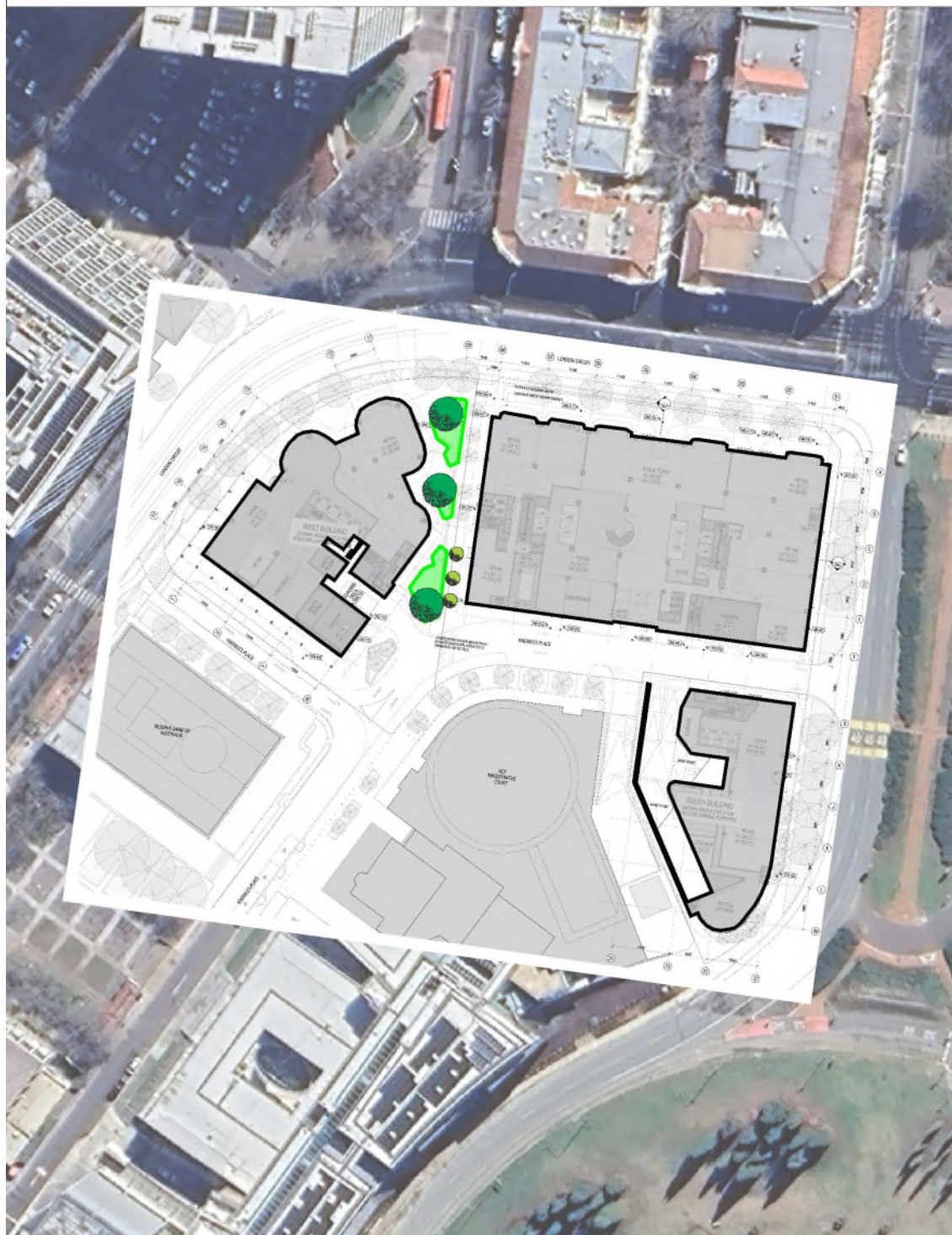
Figure 8a: Suggested Treatments – Ground Level Plan
