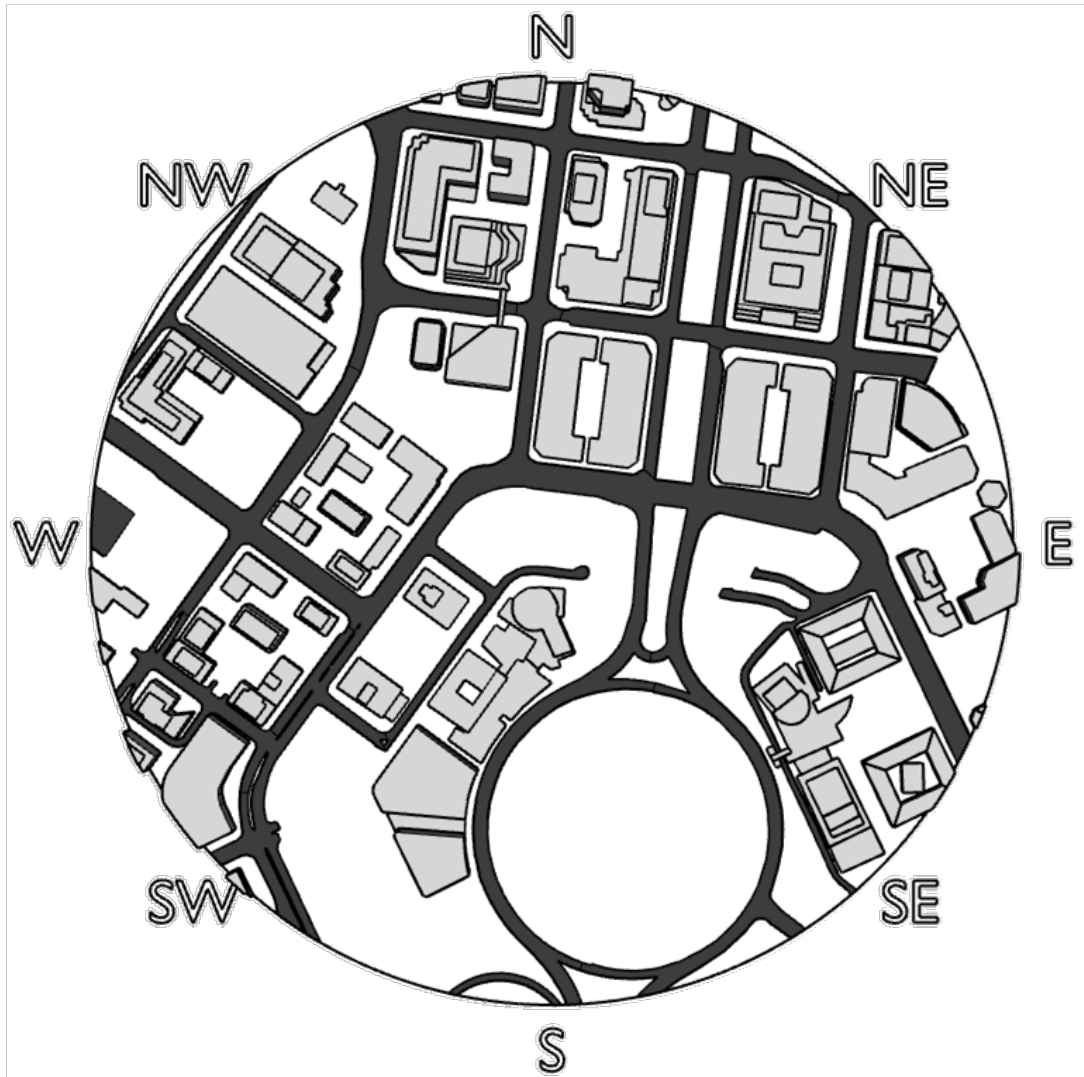
Figure 2: Proximity Model Plan - Existing Scenario
