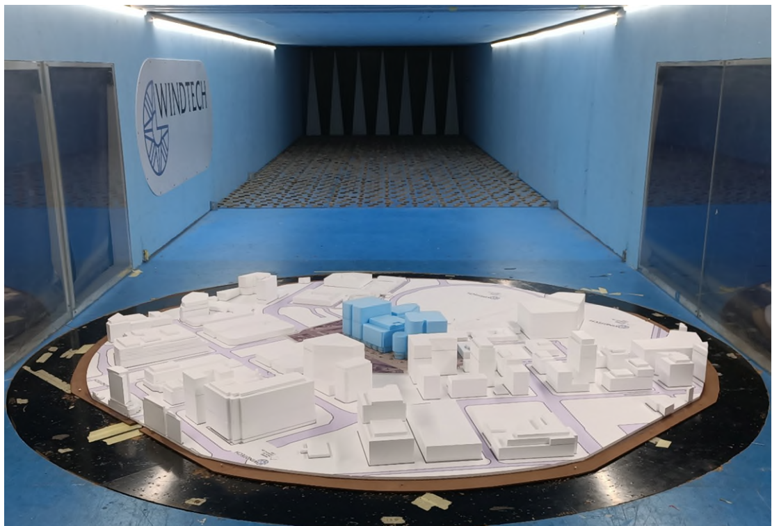
Figure 1e: Photograph of the Wind Tunnel Model (view from the north-west)
