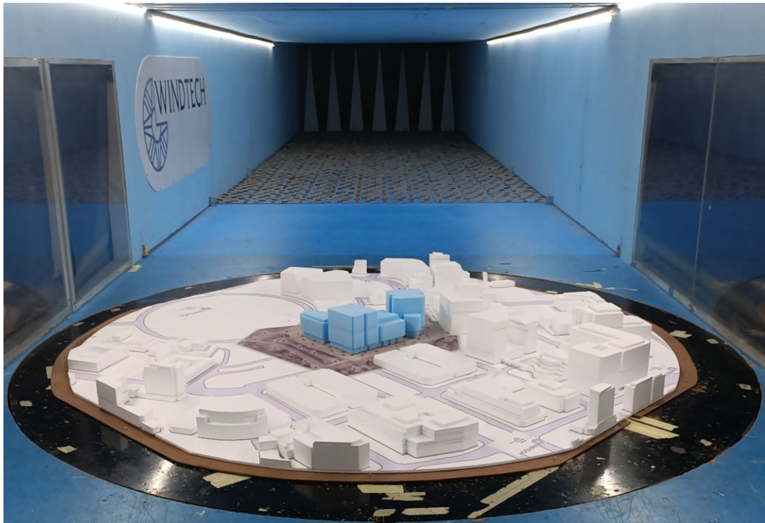
Figure 1b: Photograph of the Wind Tunnel Model (view from the north-east)
