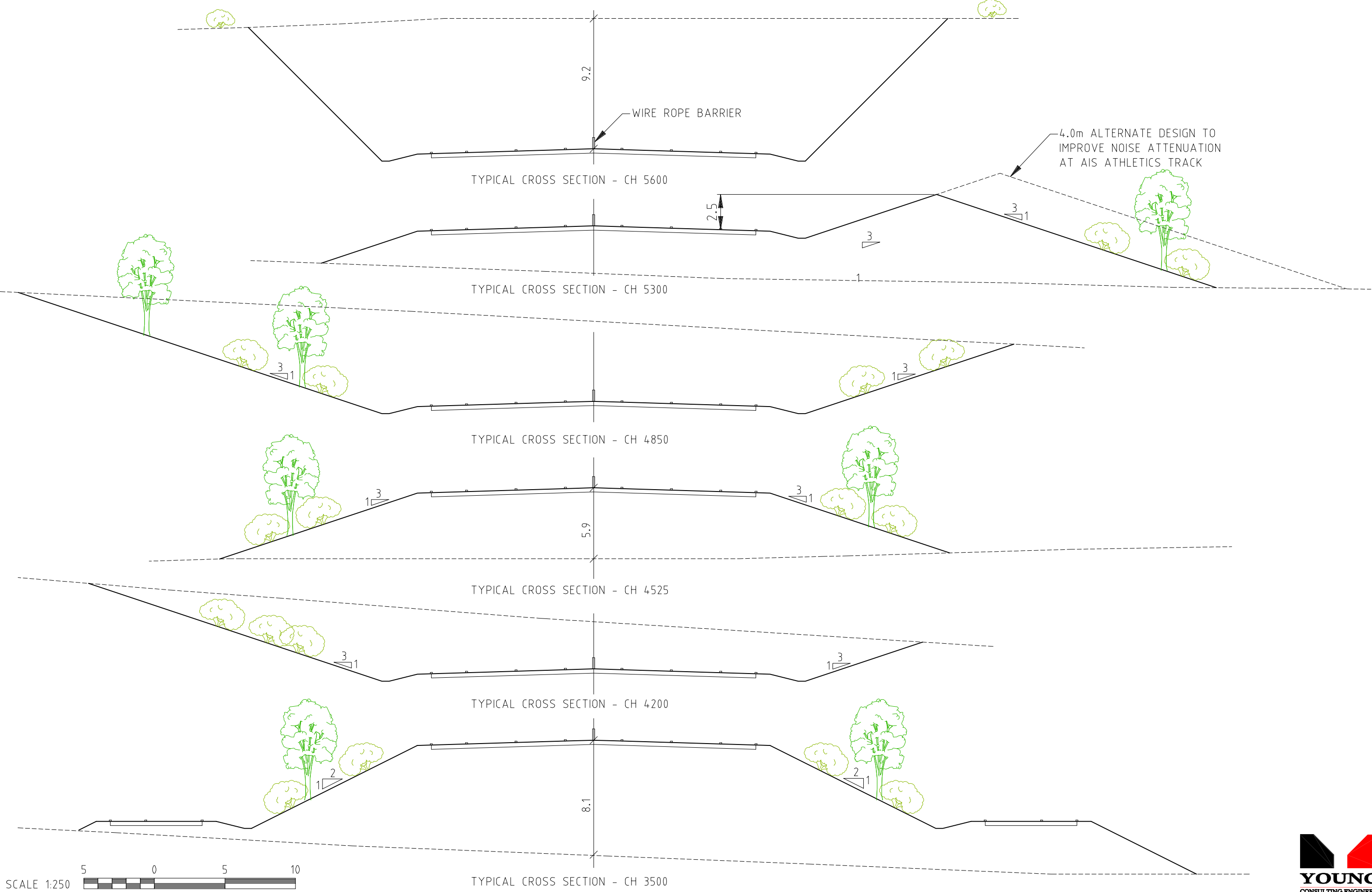
Cross Sections
