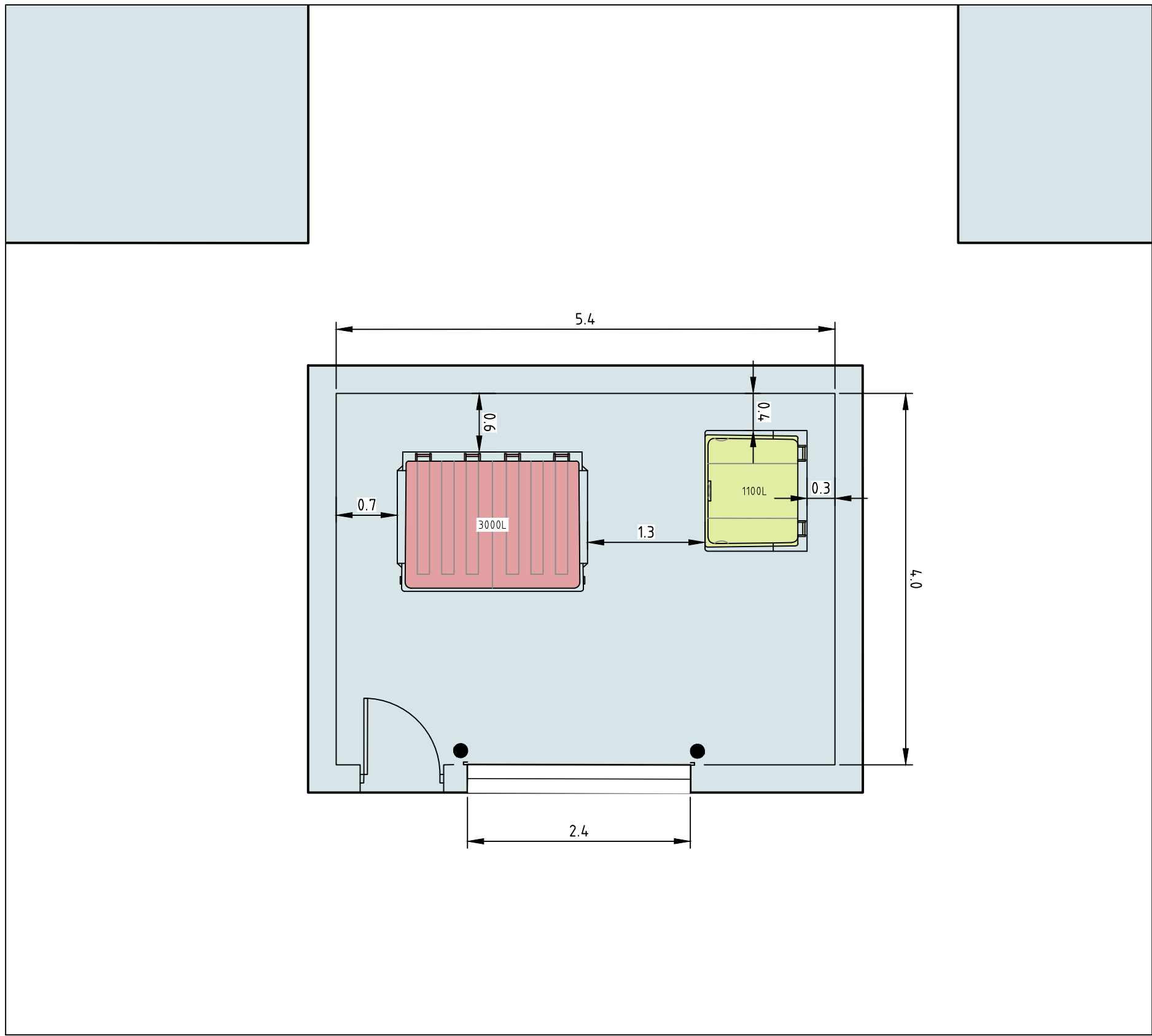
WASTE ENCLOSURE J SCALE 1:50
