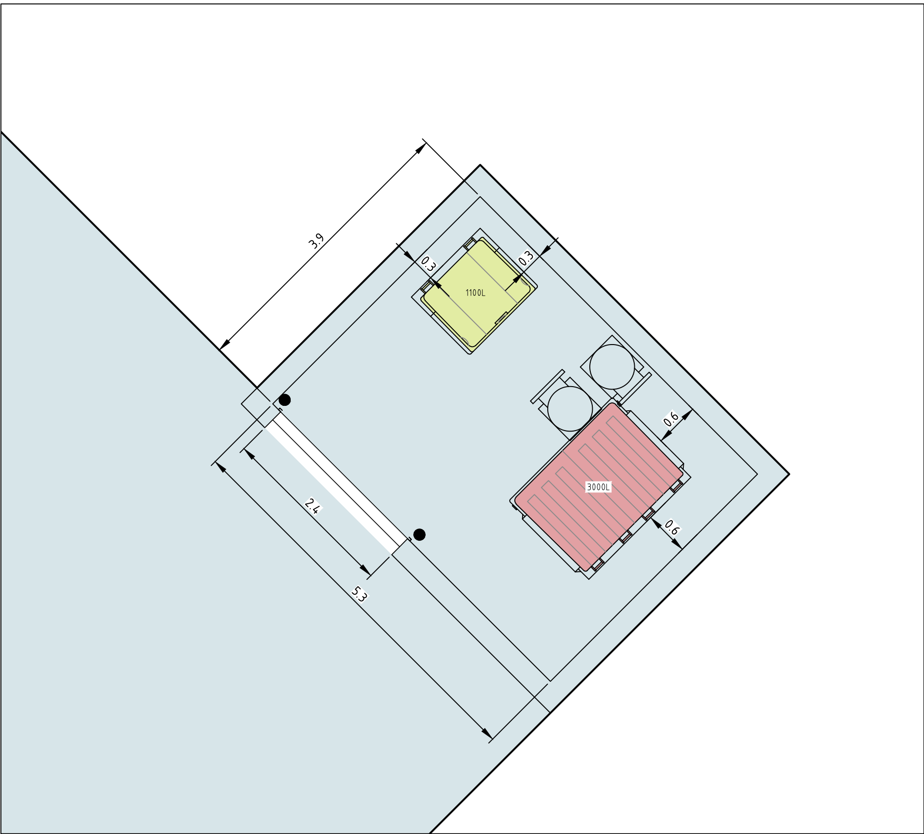
WASTE ENCLOSURE C SCALE 1:50
